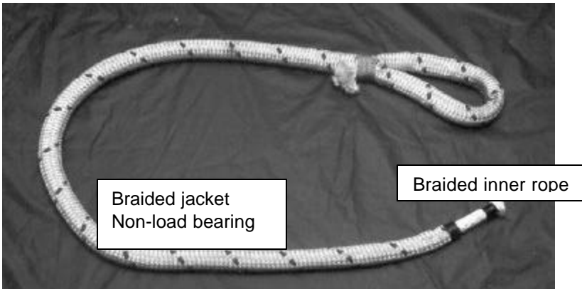
Figure 6 Jacketed Rope
