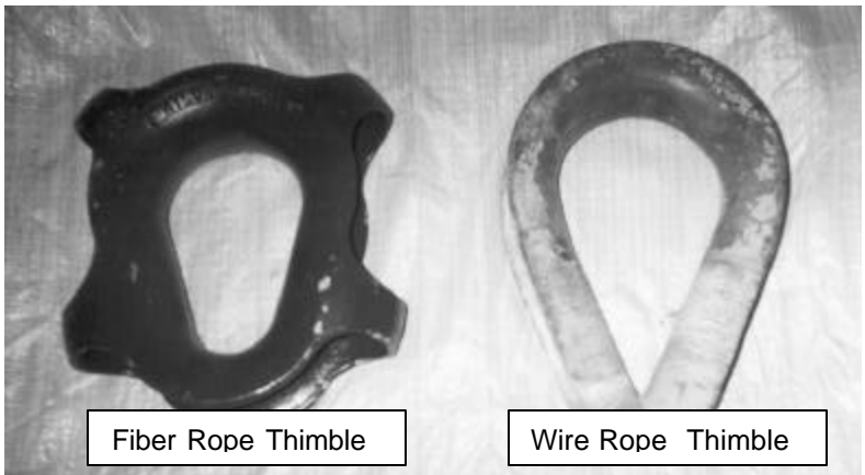
Figure 8 Thimbles
