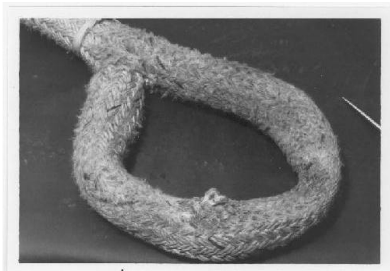
Figure D-019 Wear in Double Braid Eye Splice
